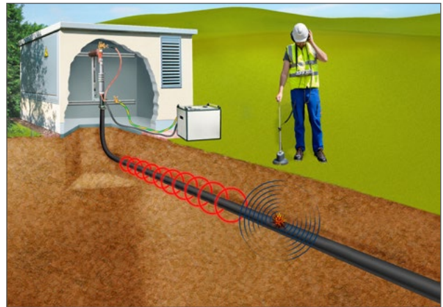
Fault location with SWG and digiPHONE + 2
